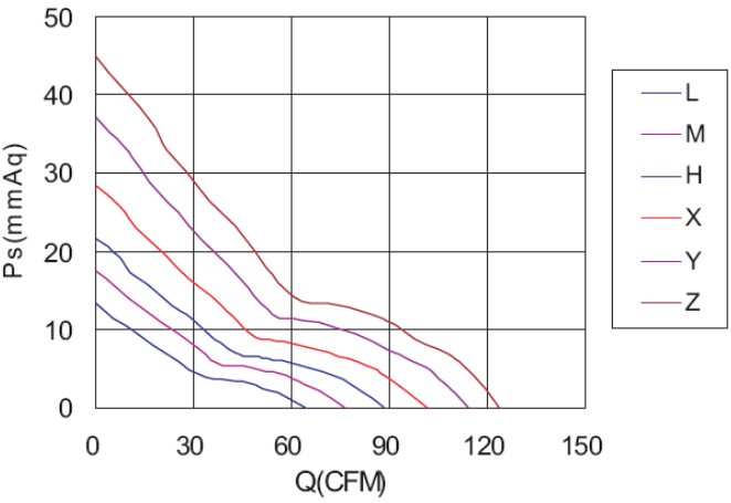
AIR FLOW/STATIC-PRESSURE
