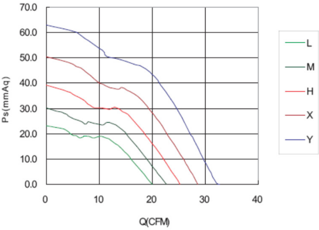
AIR FLOW/STATIC-PRESSURE
