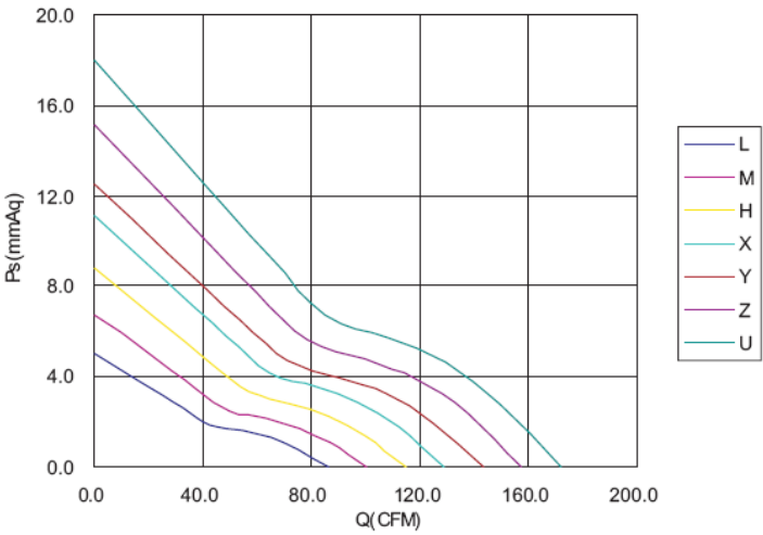
AIR FLOW/STATIC-PRESSURE
